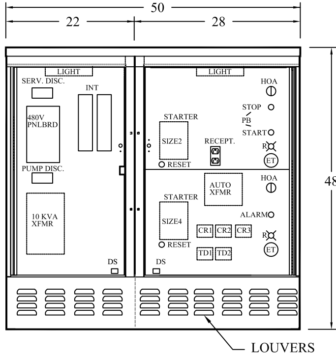
FRONT VIEW (LESS DOORS)
